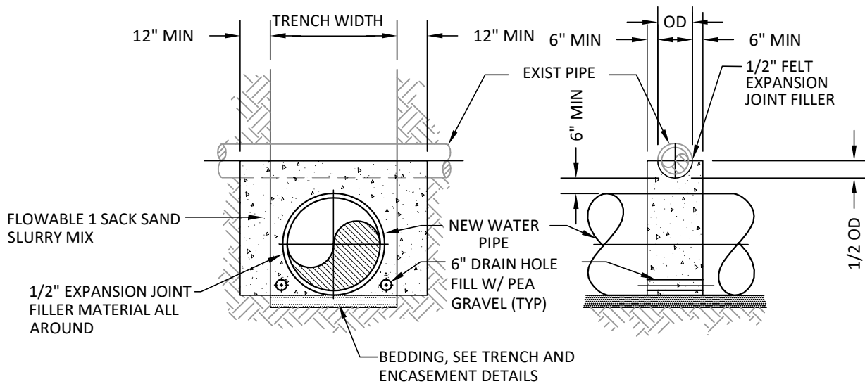
EXISTING PIPE OVER NEW WATER MAIN
