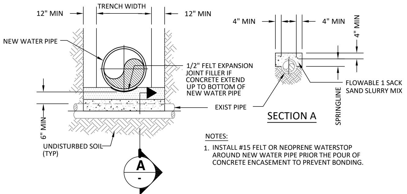
EXISTING PIPE UNDER NEW WATER MAIN
